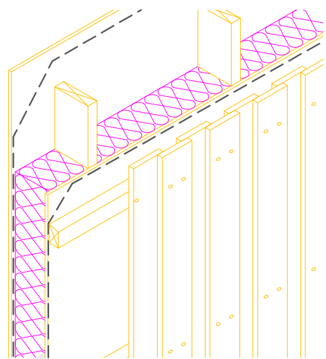
Vertical timber board on board
