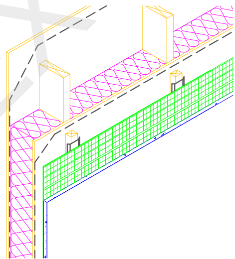
Render on metal lath
