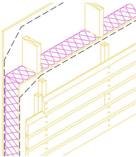
Horizontal timber boarding
